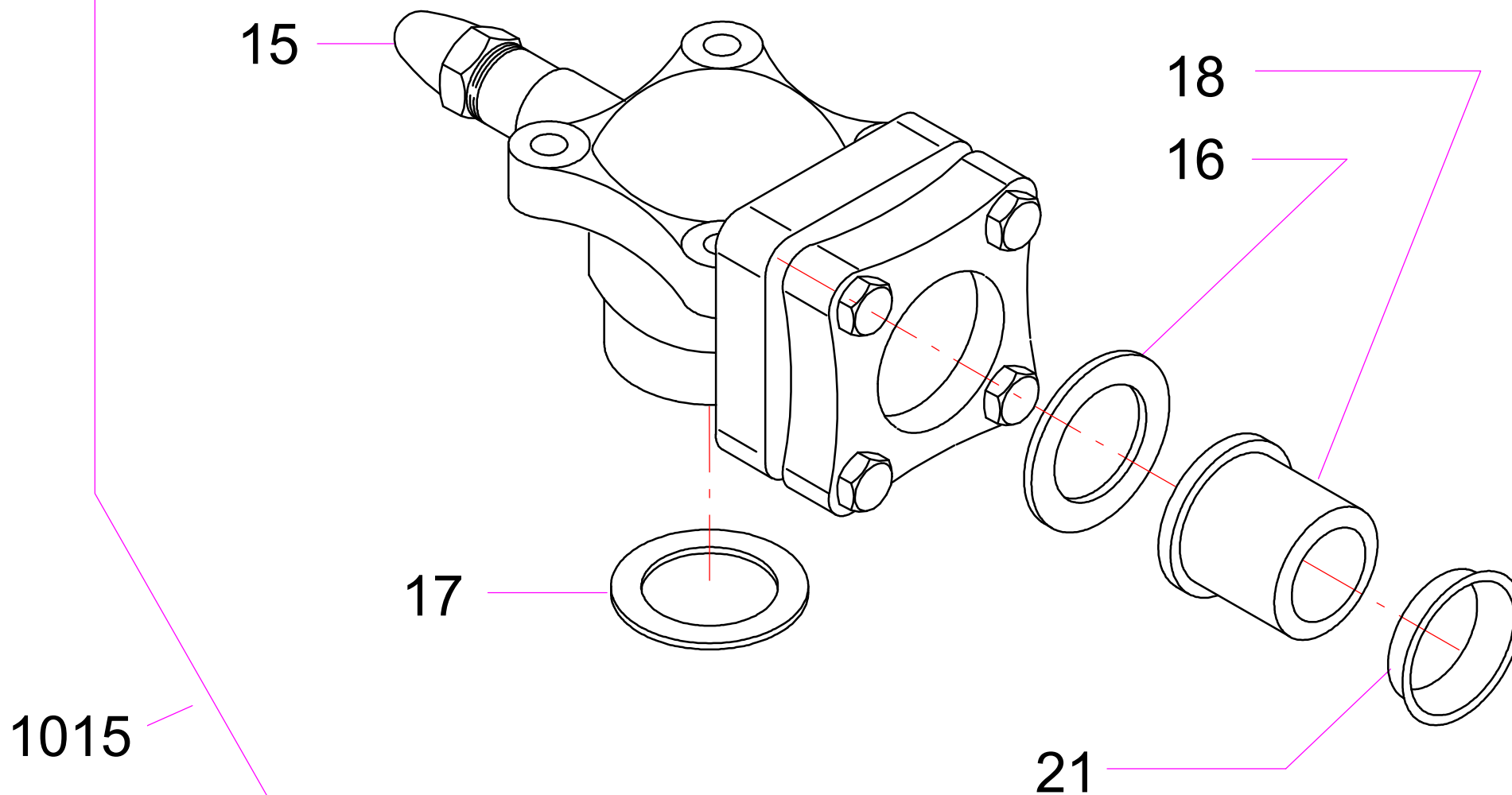
Suction shut-off valve
